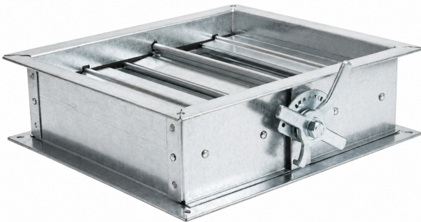
VOLUME CONTROL DAMPER (VCD) – TYPE 4
