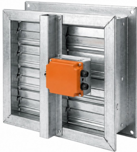
VOLUME CONTROL DAMPER (VCD) – TYPE 2
