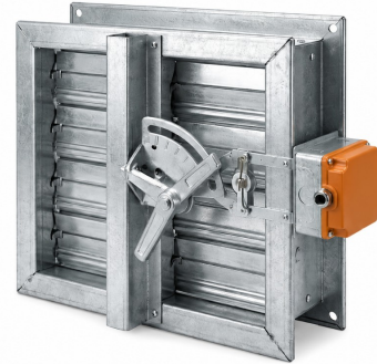
VOLUME CONTROL DAMPER (VCD) – TYPE 3
